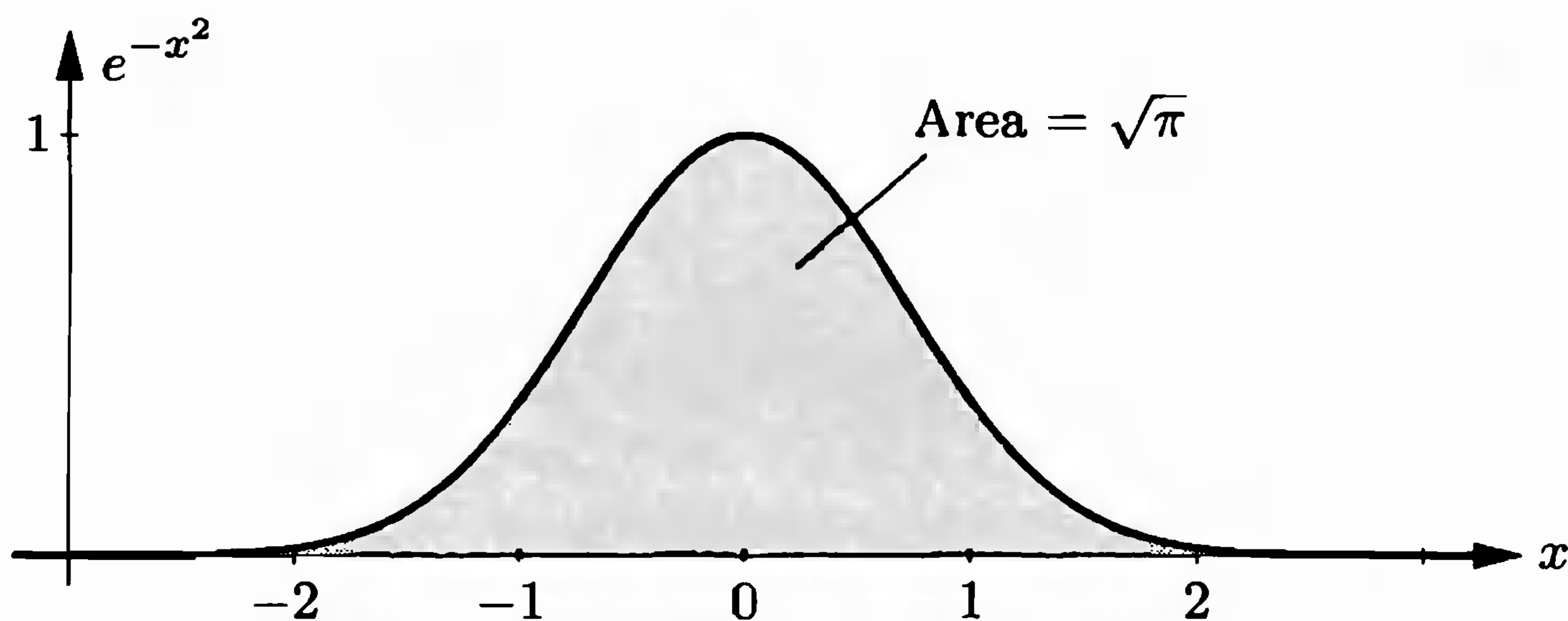
Figure B.1. The Gaussian function e^{-x^2} , whose integral from -\infty to \infty is \sqrt{\pi} .
