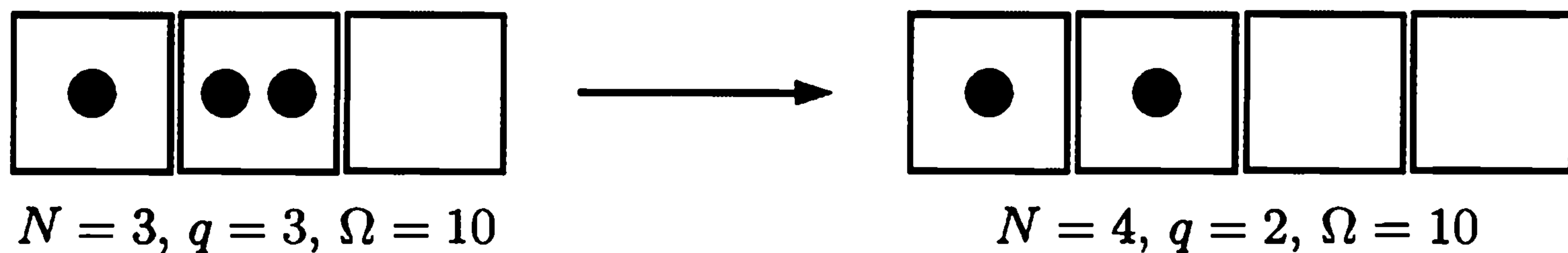
Figure 3.20. In order to add an oscillator (represented by a box) to this very small Einstein solid while holding the entropy (or multiplicity) fixed, we must remove one unit of energy (represented by a dot).
