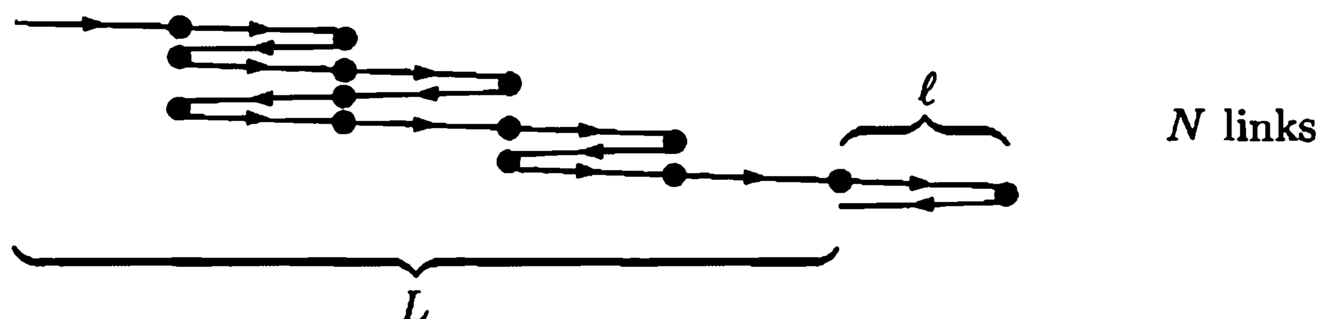
Figure 3.17. A crude model of a rubber band as a chain in which each link can only point left or right.
