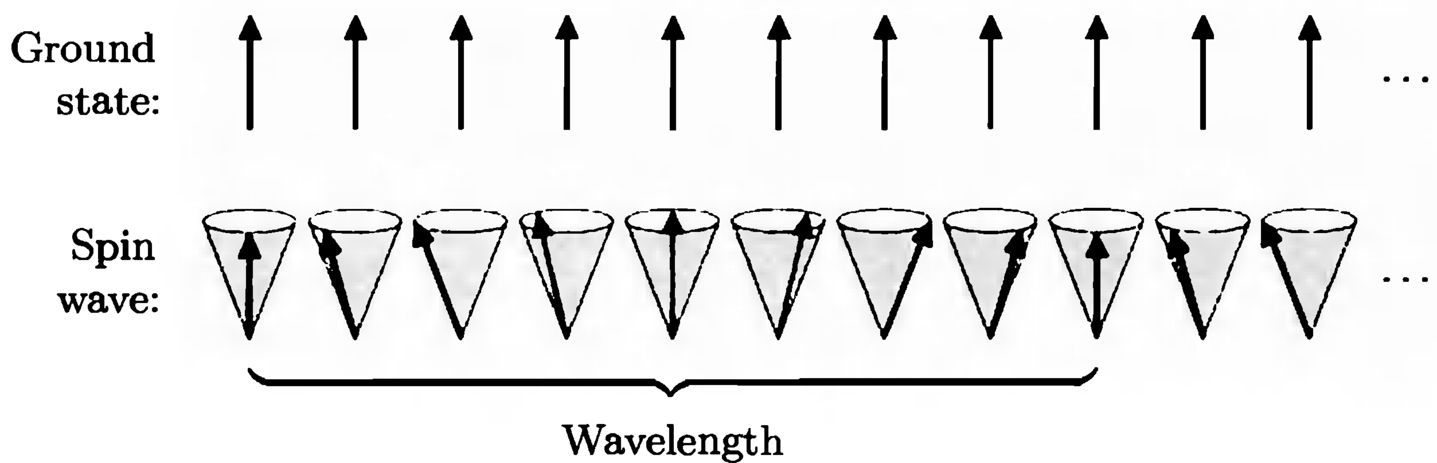
Figure 7.30. In the ground state of a ferromagnet, all the elementary dipoles point in the same direction. The lowest-energy excitations above the ground state are spin waves , in which the dipoles precess in a conical motion. A long-wavelength spin wave carries very little energy, because the difference in direction between neighboring dipoles is very small.
