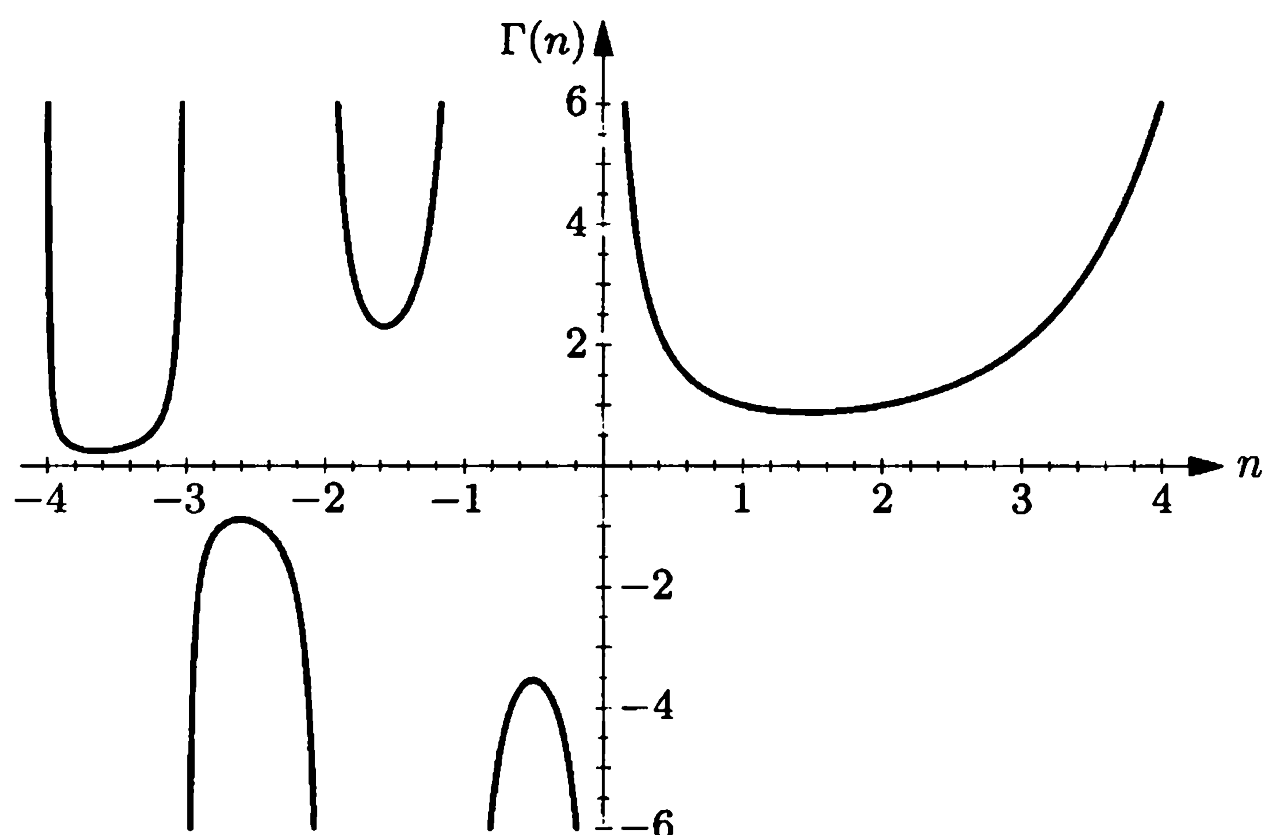
Figure B.3. The gamma function, \Gamma(n) . For positive integer arguments, \Gamma(n) = (n - 1)! . For positive nonintegers, \Gamma(n) can be computed from equation B.12, while for negative nonintegers, \Gamma(n) can be computed from equation B.14.
