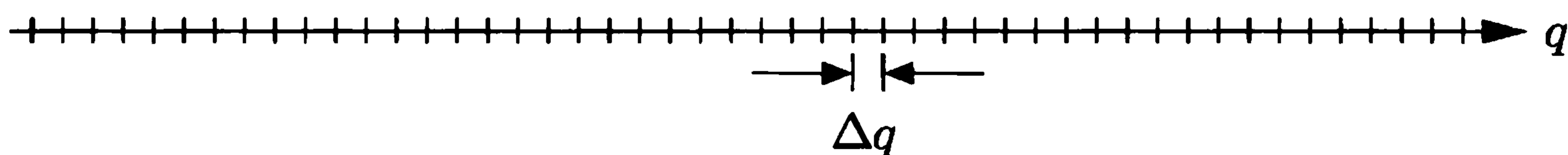
Figure 6.8. To count states over a continuous variable q , pretend that they're discretely spaced, separated by \Delta q .
