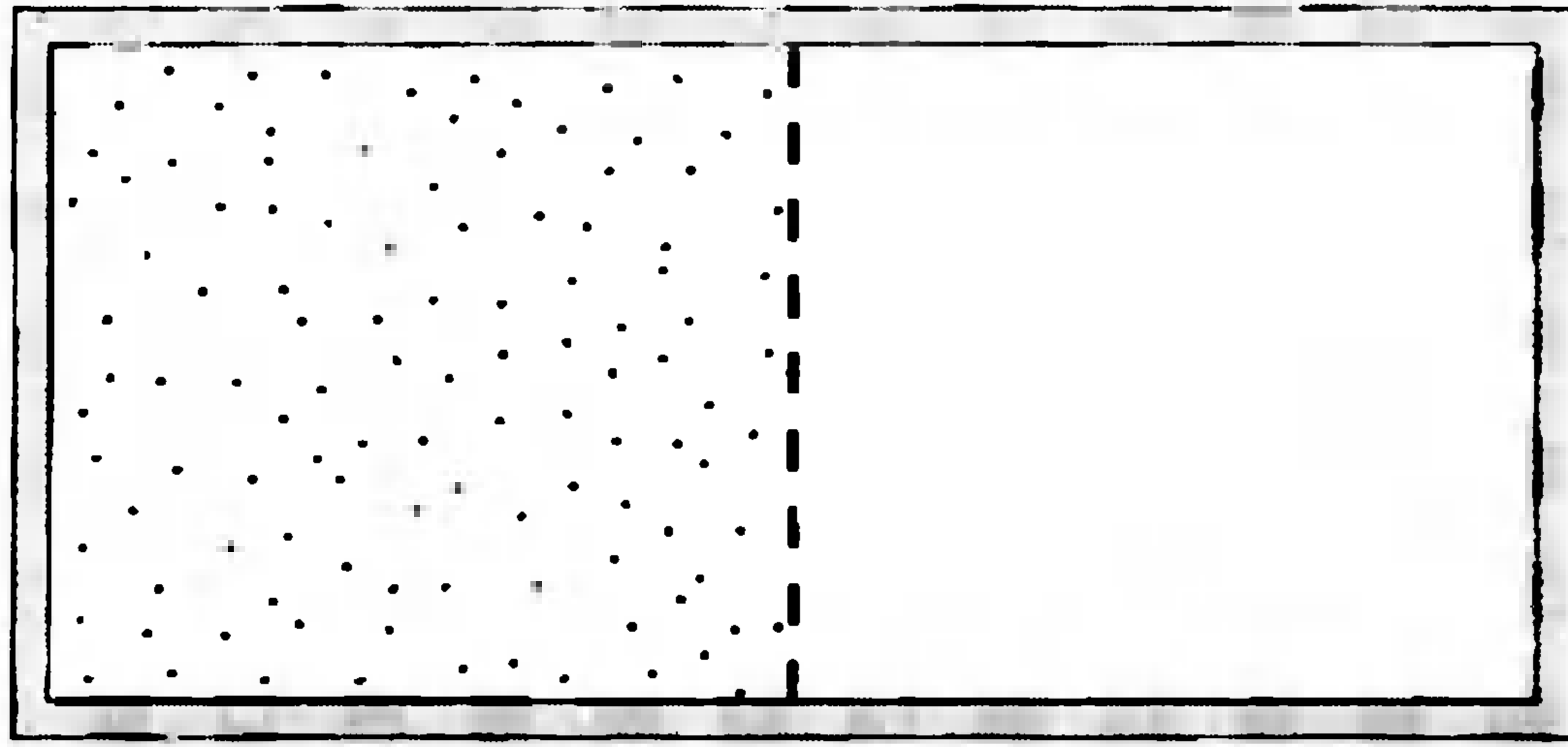
Figure 2.13. A very unlikely arrangement of gas molecules.
