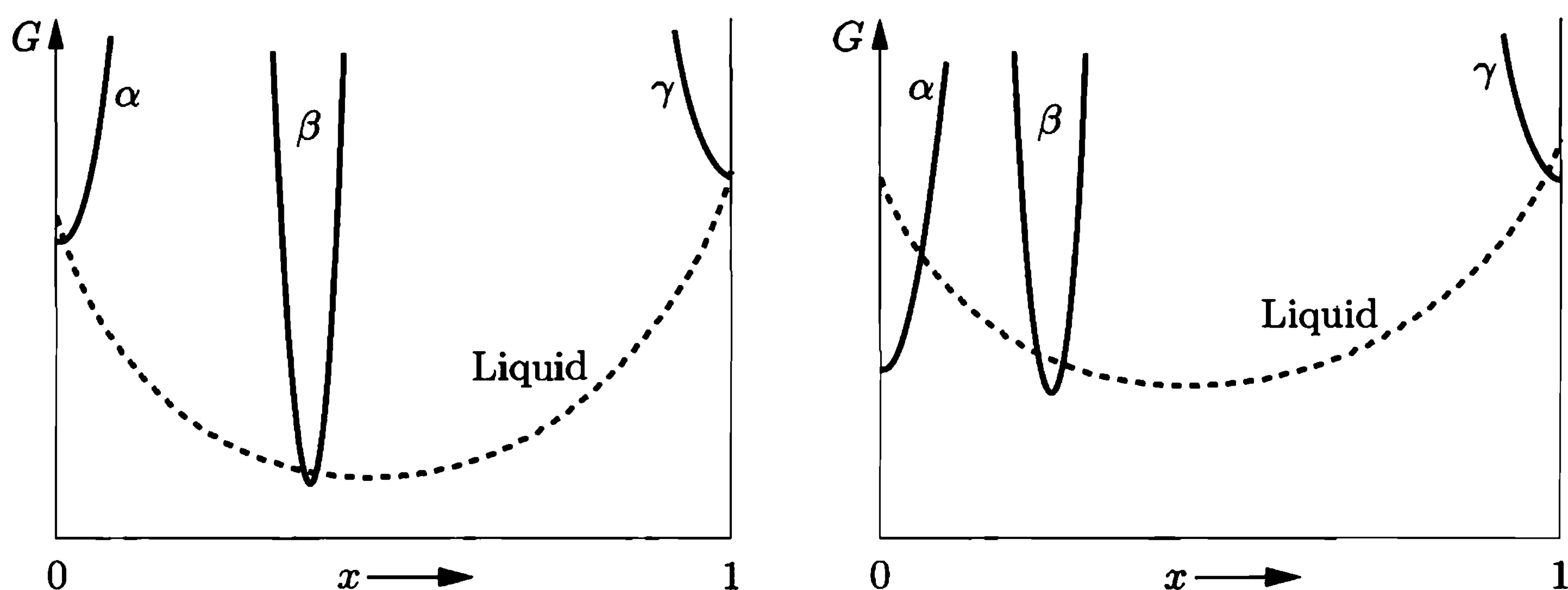
Figure 5.35. Free energy diagrams for Problems 5.71 and 5.72.
